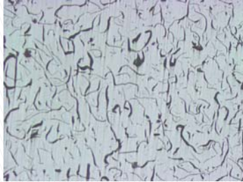
Microstructure of grey iron
