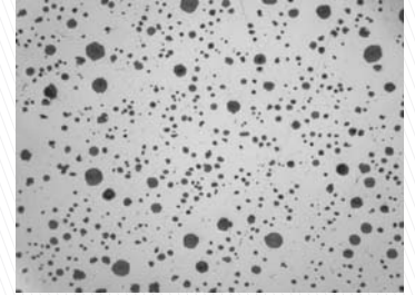
Microstructure of ductile iron
